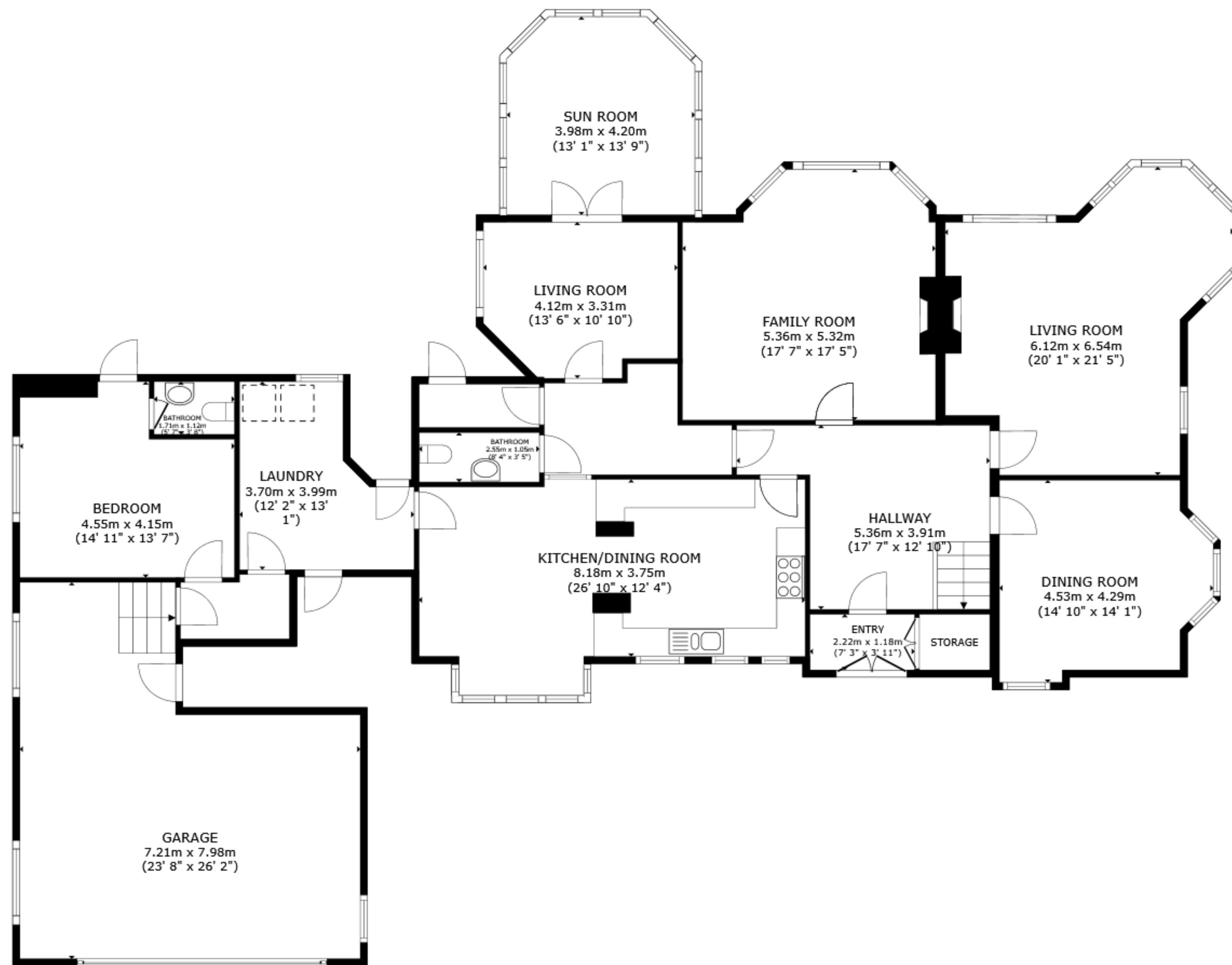
FLOOR 1
